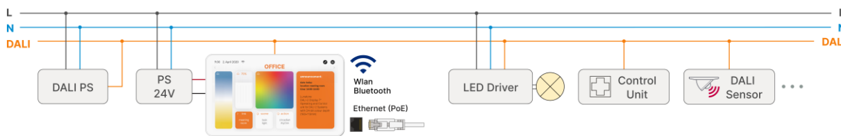
Figure 1 Typical Application
