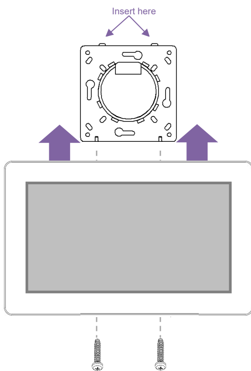
Figure 2 Mounting
